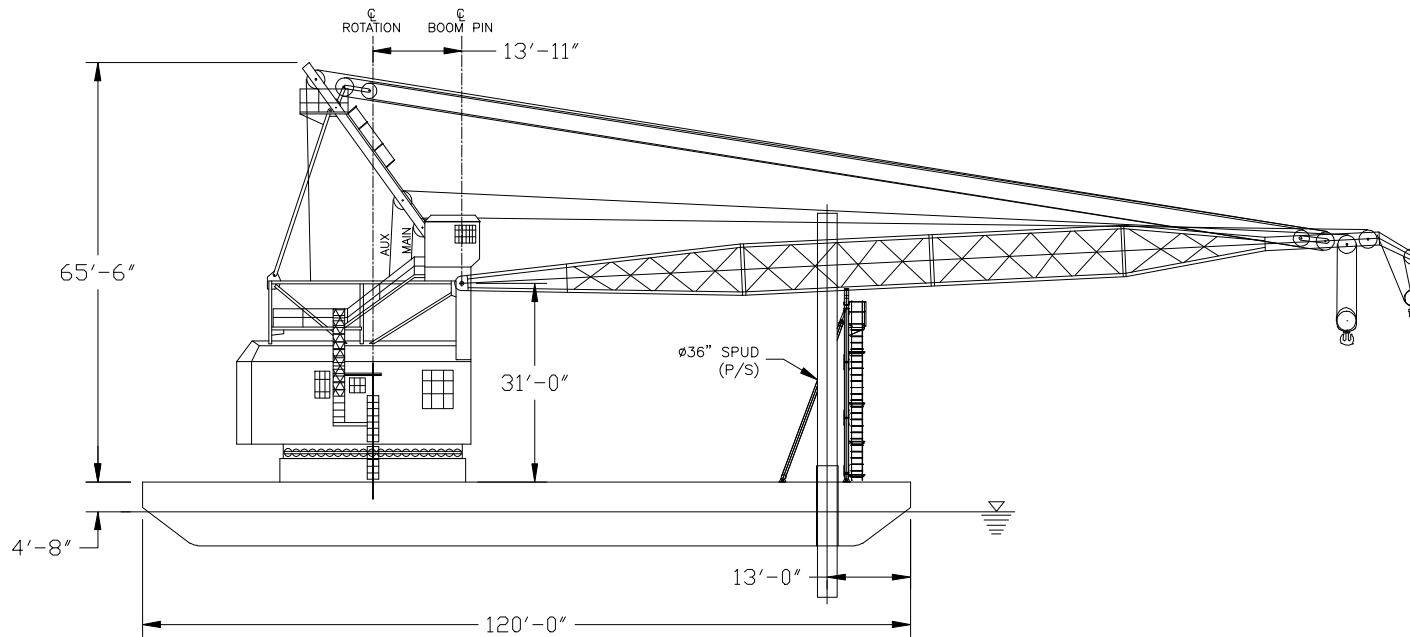
OUTBOARD PROFILE
